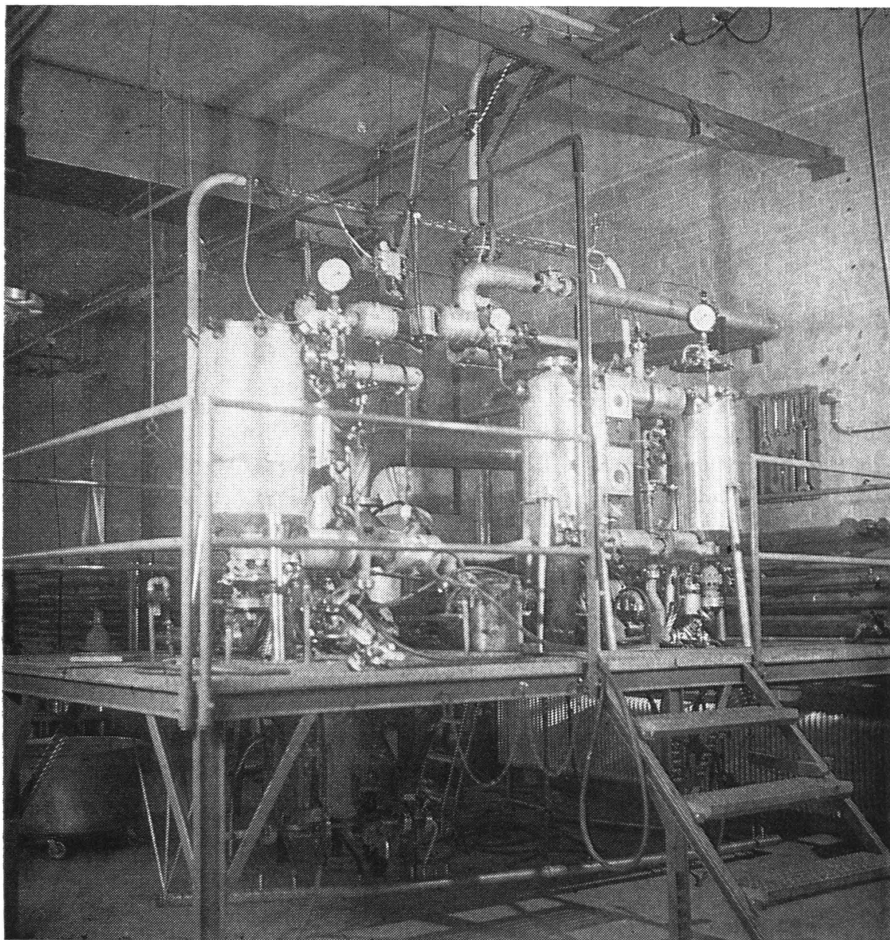
A view of the pilot cooking equipment in the pilot plant hall of the Forest Products Department.
