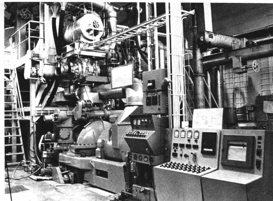
The thermomechanical pulping station, with Bauer 412 double-disk refiner (1600 kW).
